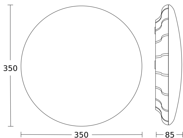
Dimension Drawing
